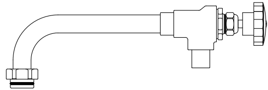
5071 10" CONTROL SWING SPOUT
