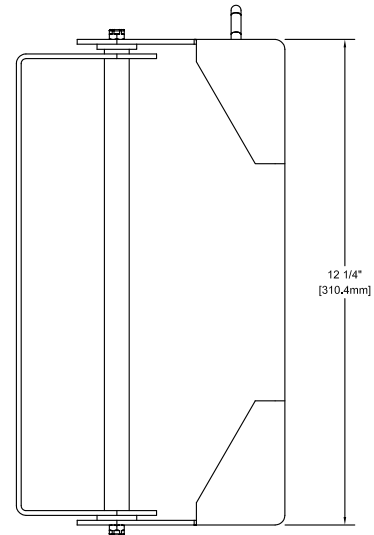
SIDE VIEW
