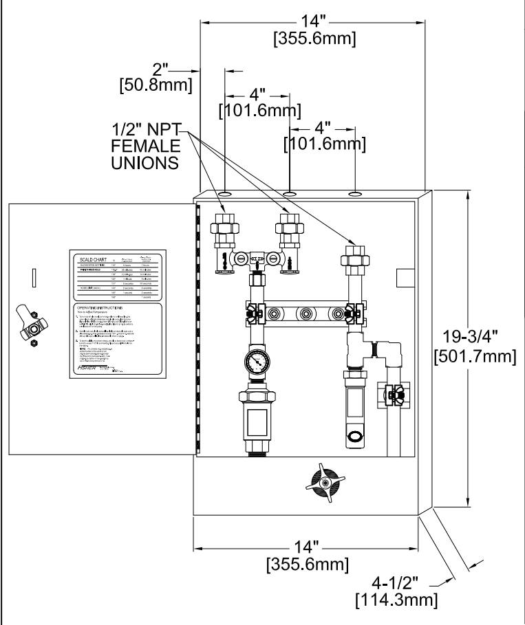
RECESSED MOUNTING
