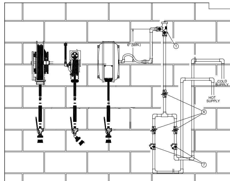
EXPOSED PIPES
