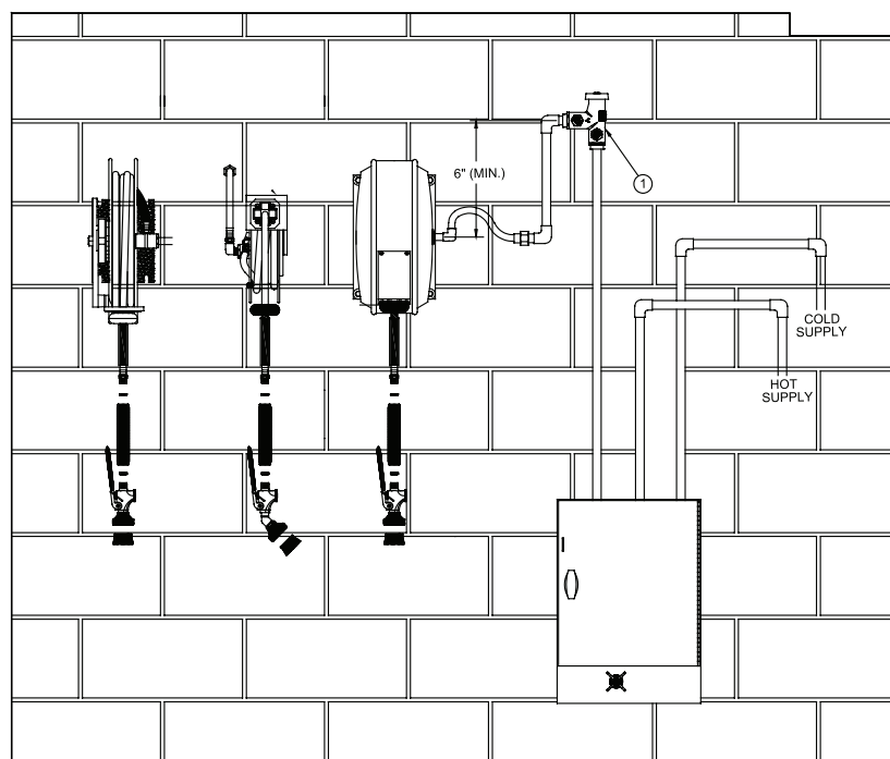
EXPOSED PIPES
