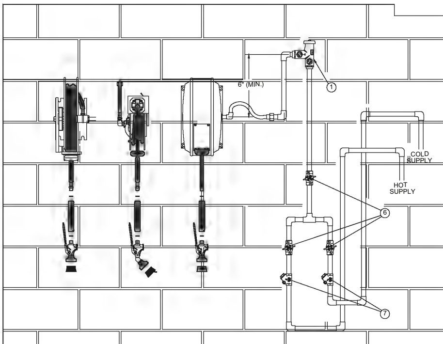
EXPOSED PIPES
